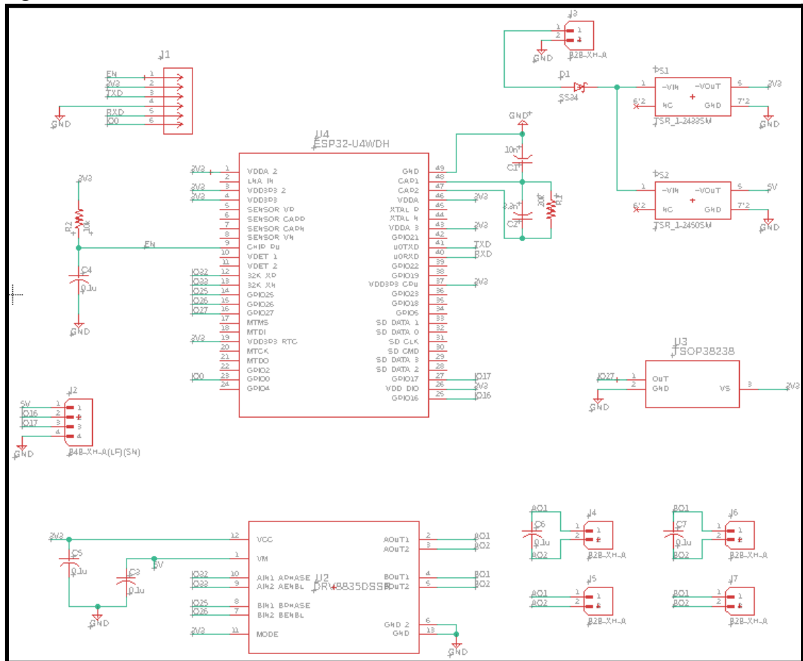
Figure 6.1.1 - Car PCB Schematic
